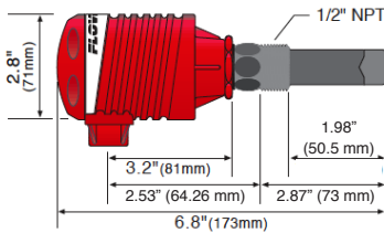
Dimensions (w/ long sensor)
