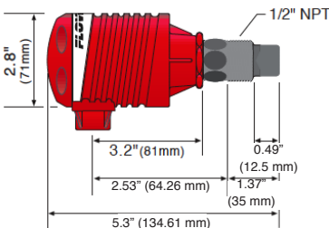
Dimensions (w/ short sensor)
