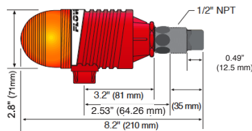
Dimensions (w/ short sensor & strobe light)
