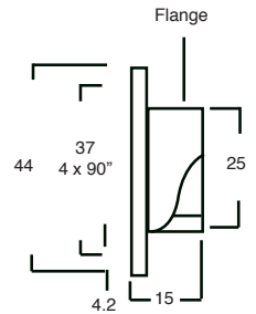
Mounting Flange
