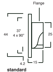
Mounting Flange
